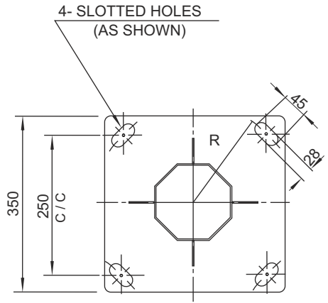
BASE PLATE DETAIL SIZE: 350x350x15 THK.
