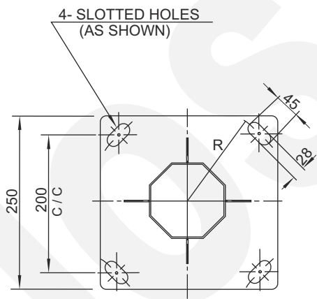
BASE PLATE DETAIL SIZE: 250x250x10 THK.
