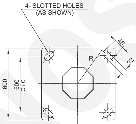
BASE PLATE DETAIL SIZE: 600x600x30 THK.
