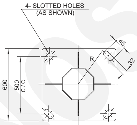
BASE PLATE DETAIL SIZE: 500x500x30 THK.
