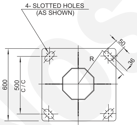
BASE PLATE DETAIL SIZE: 600x600x25 THK.
