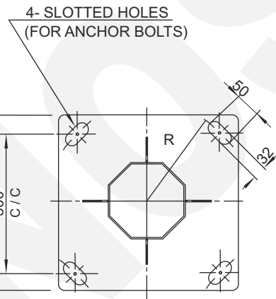
BASE PLATE DETAIL SIZE: 600x600x25 THK.
