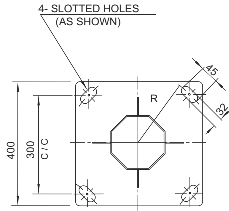
BASE PLATE DETAIL SIZE: 400x400x20 THK.
