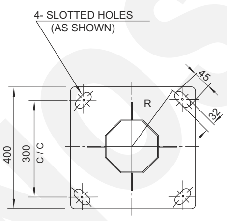
BASE PLATE DETAIL SIZE: 400x400x20 THK.
