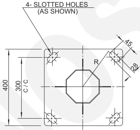
BASE PLATE DETAIL SIZE: 400x400x15 THK.
