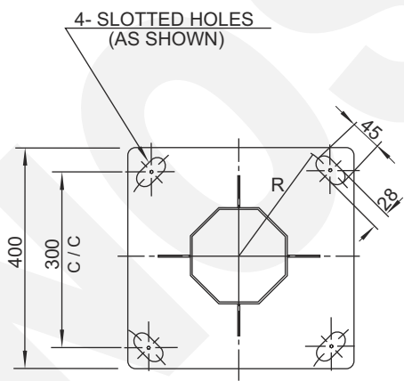
BASE PLATE DETAIL SIZE: 400x400x15 THK.
